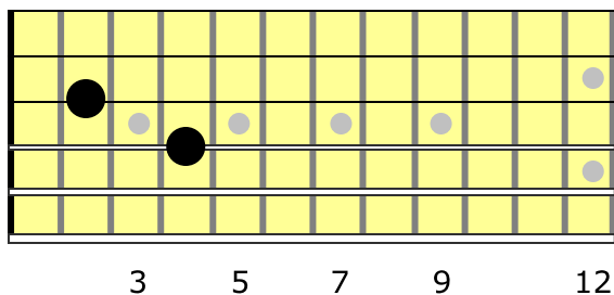
F#m
